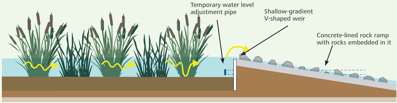
Figure 16. Recommended rock-ramp design to provide fish passage in and out of wetlands and between cells. The water level control weir should be broad, with a shallow V shaped profile (5-10° lateral slope). The rock ramp should have a low gradient (<1:10 for fall heights of ≤1m, <1:15 for heights of 1-4m; and 1:30 for weakly-swimming species such as inanga). Mixed grade rocks (150-200mm diameter) should be securely embedded in the concrete-lined ramp to approximately half their depth to create zones of calmer flow at the margins and a low-flow channel at the centre suitable for the movement of fish. A low level pipe is recommended to enable control of water level during initial plant establishment or wetland maintenance. A swivelling elbow or standpipe can be added to adjust water levels during these periods. This pipe should be capped once the plants are sufficiently grown to cope with deeper water levels (3-4 months).
